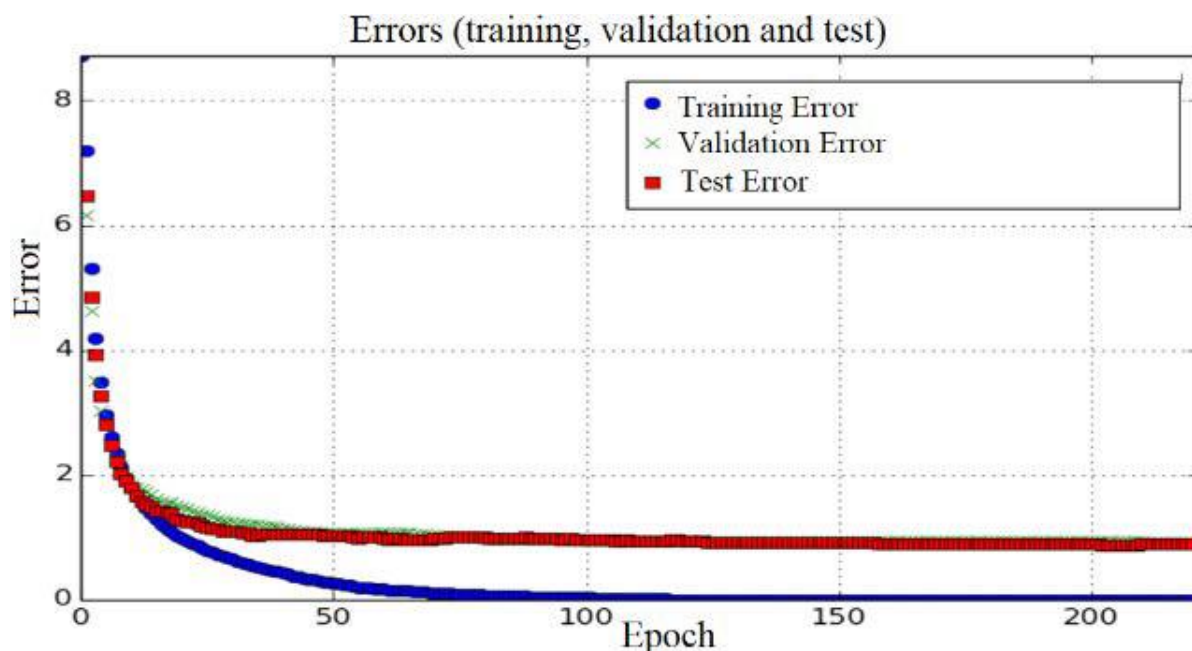
Figure 1. Training, validation and test errors.
