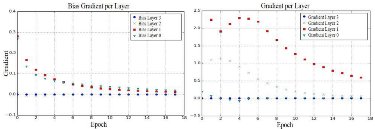
Figure 2. Gradient behaviour per layer, left gradient of bias, right gradient of weights.
