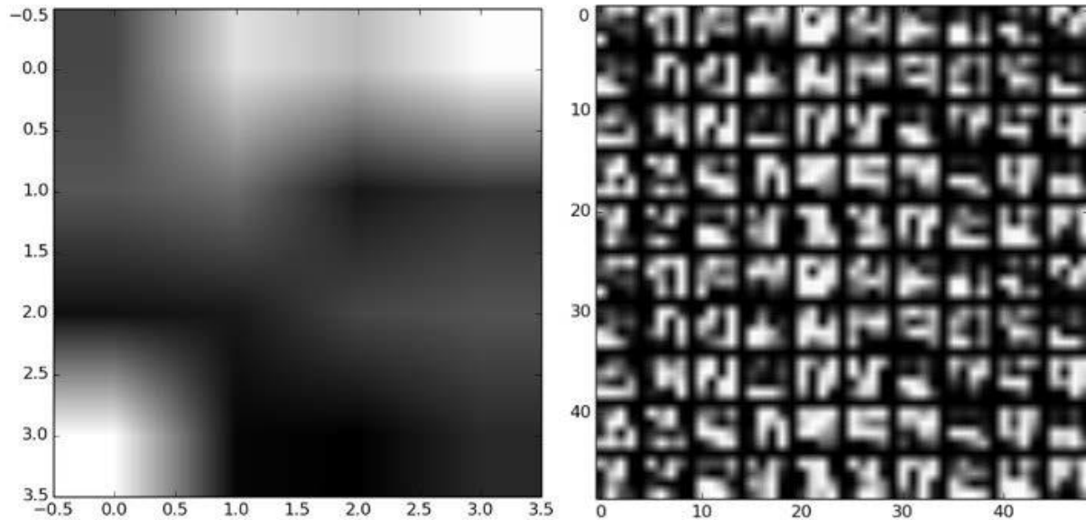
Figure 4. Images obtained after the second convolution layer. Left: simple image, right: mosaic with different and random filters.
